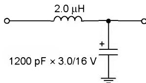
Figure 19. Input Filter
