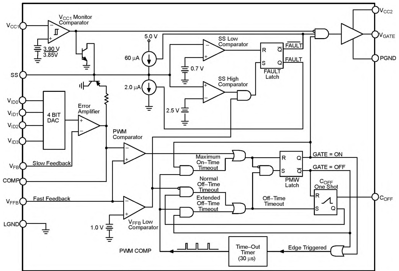
Figure 2. Block Diagram
