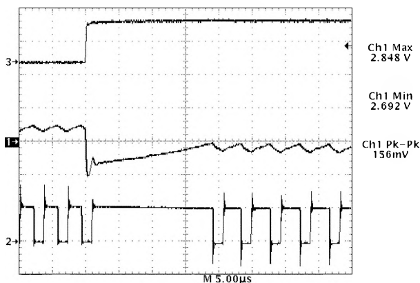
Figure 9. CS5151H Demonstration Board Response to a 0.5 to 13 A Load Pulse (Output Set for 2.8 V)
