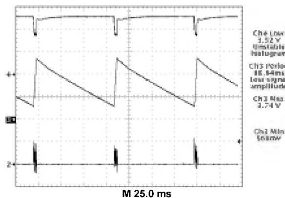
Figure 12. CS5151H Demonstration Board Hiccup Mode Short Circuit Protection. Gate Pulses are Delivered While the Soft Start Capacitor Charges, and Cease During Discharge
