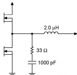
Figure 18. Filter Components
