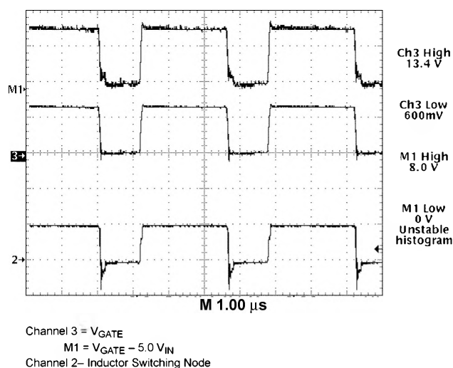
Figure 17. CS5151H Gate Drive Waveforms Depicting Rail to Rail Swing
