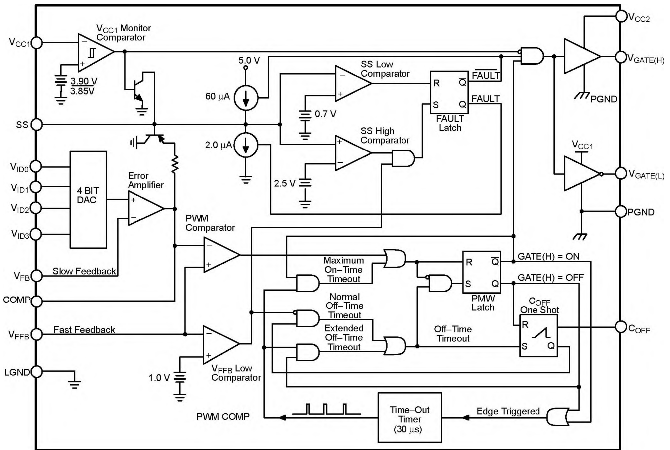
Figure 2. Block Diagram
