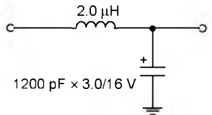
Figure 21. Input Filter
