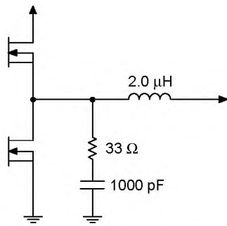
Figure 20. Filter Components
