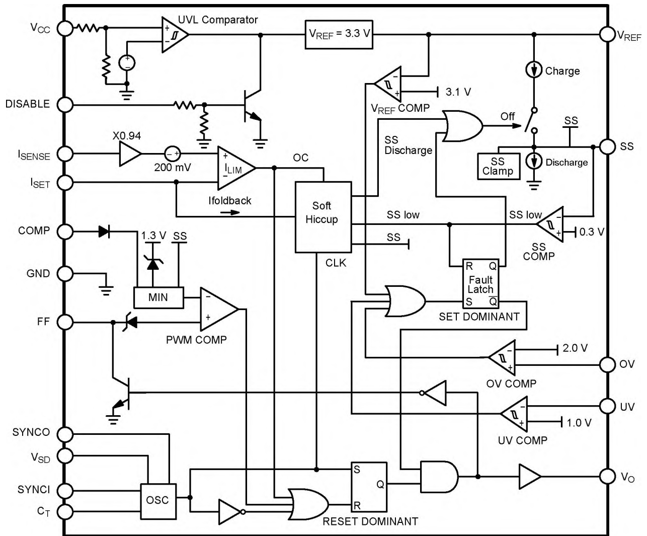
Figure 2. Block Diagram
