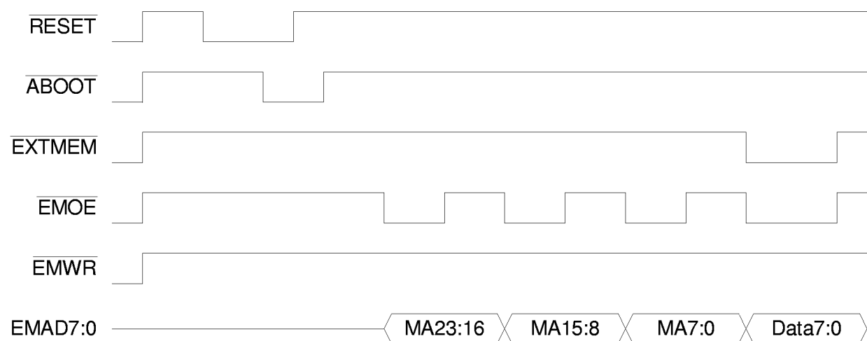
Figure 23. Autoboot Timing Diagram
