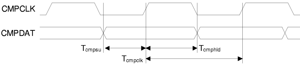
Figure 2. Serial Compressed Data Timing
