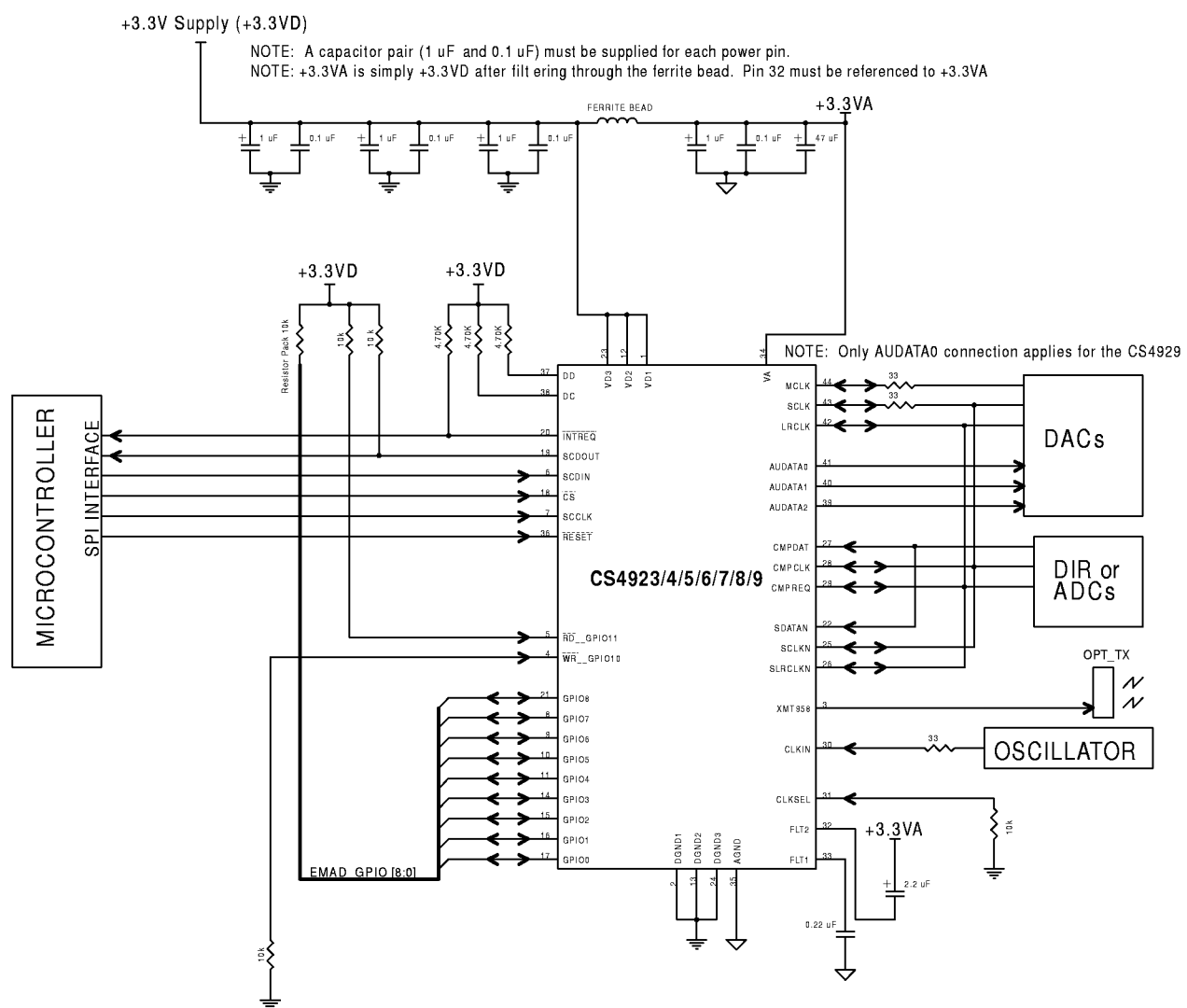
Figure 15. SPI Control
