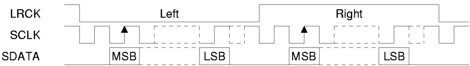
Figure 24. I²S Format
