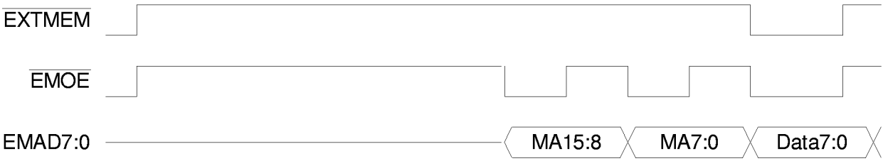
Figure 22. Run-Time Memory Access
