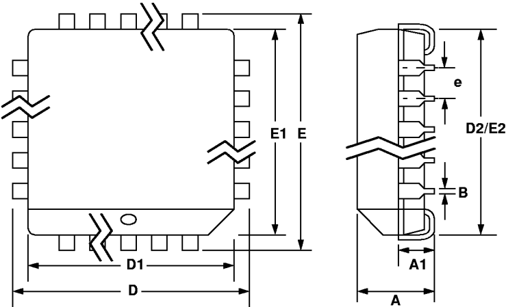
44L PLCC PACKAGE DRAWING
