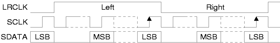
Figure 26. Right Justified
