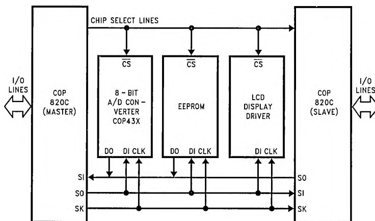
FIGURE 8. MICROWIRE/PLUS Application
