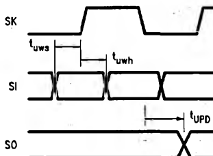
FIGURE 2. MICROWIRE/PLUS Timing
