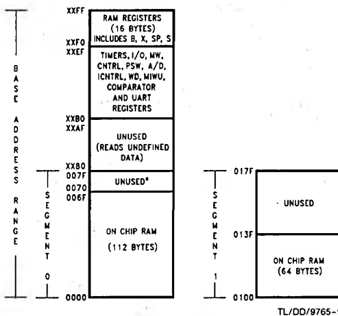
FIGURE 4. RAM Organization
