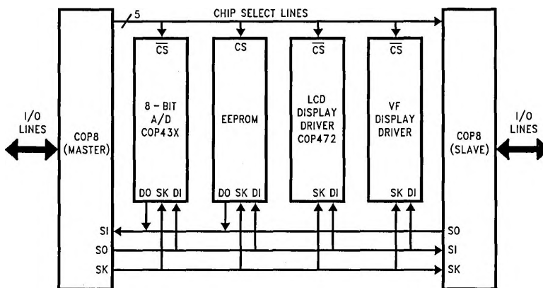
FIGURE 15. MICROWIRE/PLUS Application
