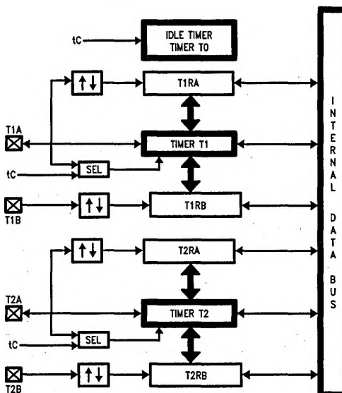
FIGURE 7. Timers
