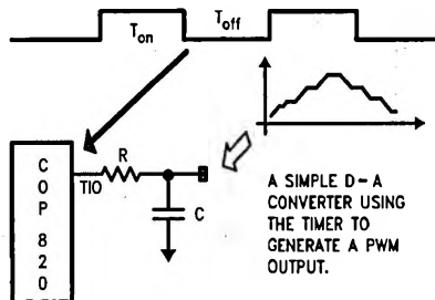
FIGURE 11. Timer Application
