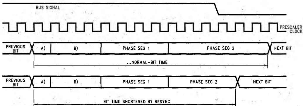
FIGURE 33. Resynchronization 2
