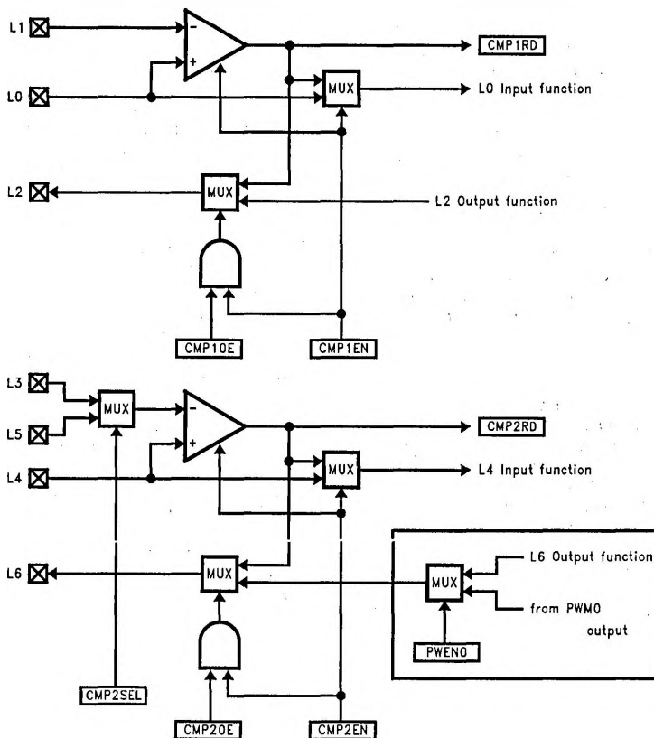
FIGURE 34. Comparator Block
