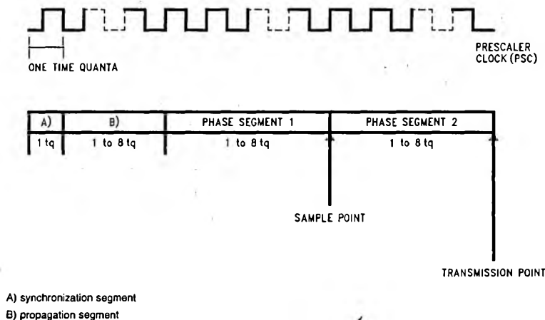
FIGURE 31. Bit Timing
