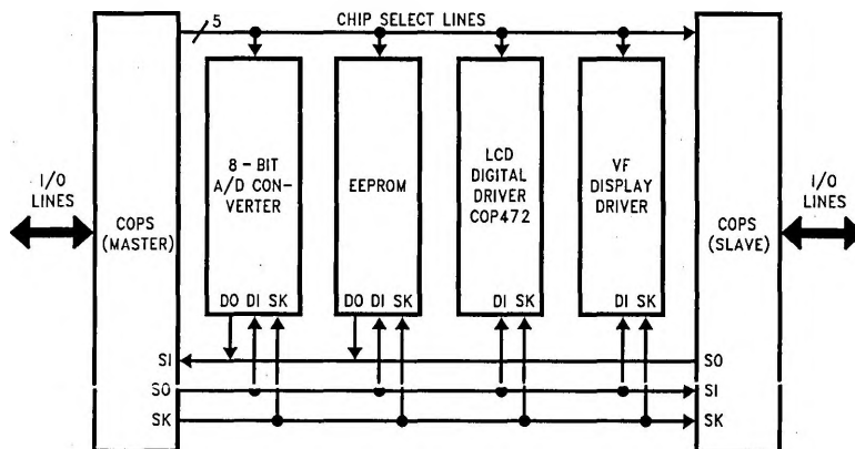
FIGURE 36. MICROWIRE/PLUS Application
