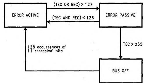
FIGURE 30. CAN Bus States
