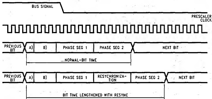
FIGURE 32. Resynchronization 1
