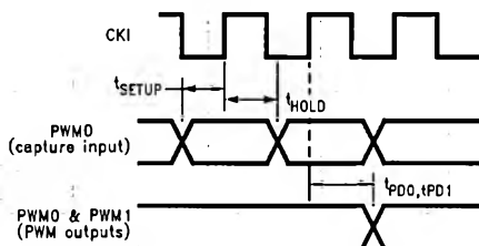
FIGURE 4. PWM/CAPTURE Timer Input/Output Timing Diagram
