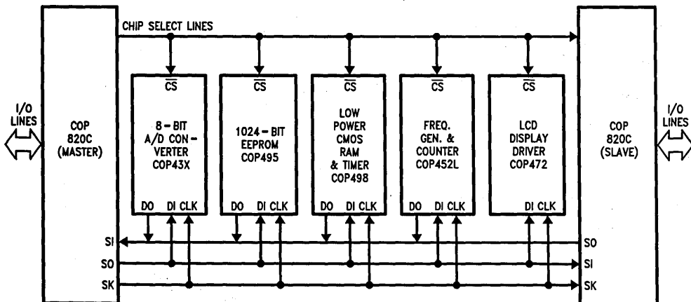
FIGURE 8. MICROWIRE/PLUS Application
