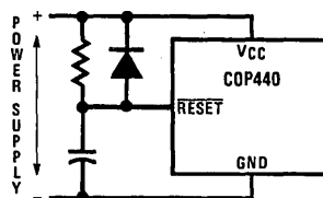
FIGURE 8. Power-Up Clear Circuit
