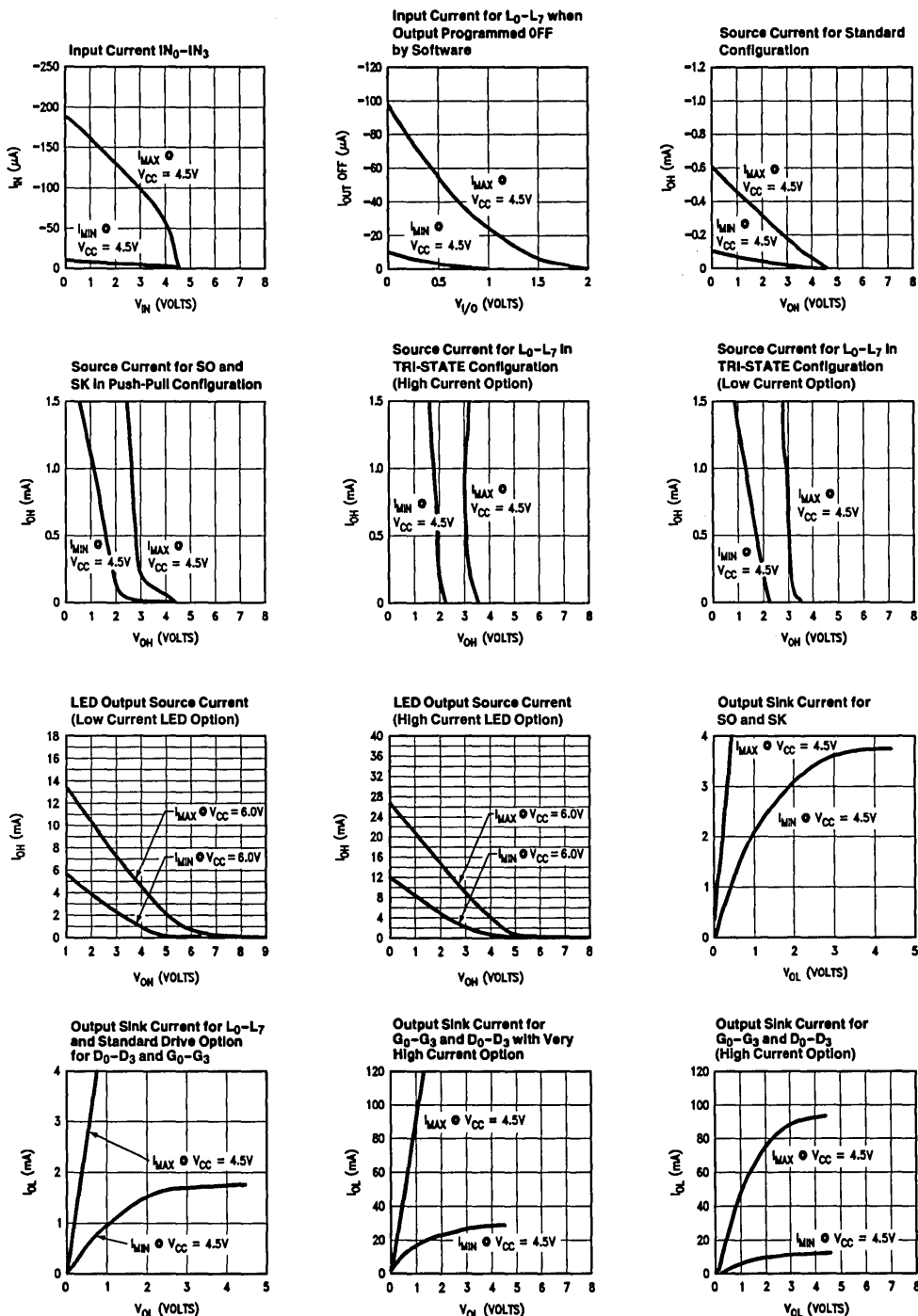
FIGURE 7. COP320L/DOP321L/COP322L Input/Output Characteristics
