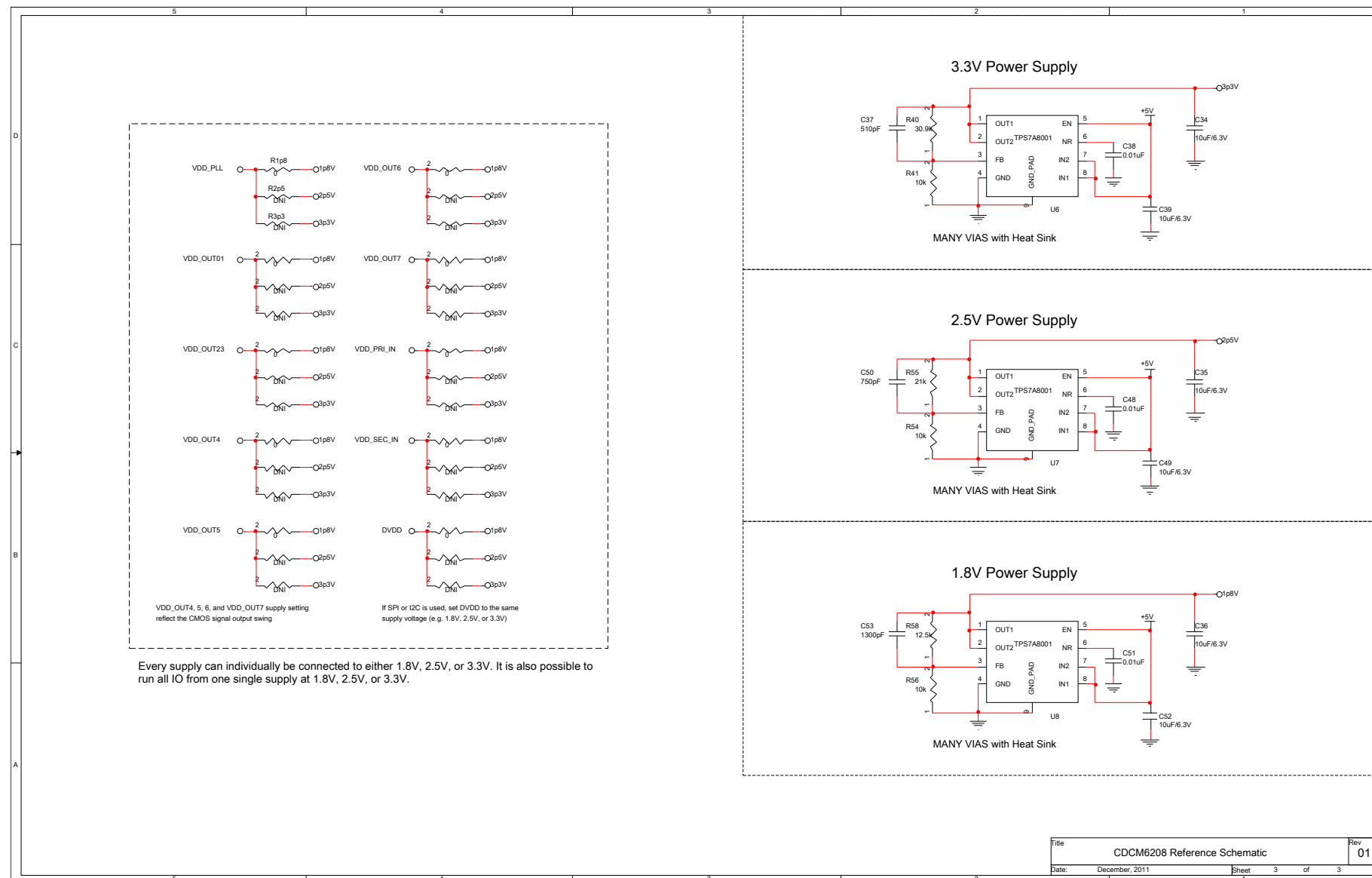
Figure 56. Schematic page 3
