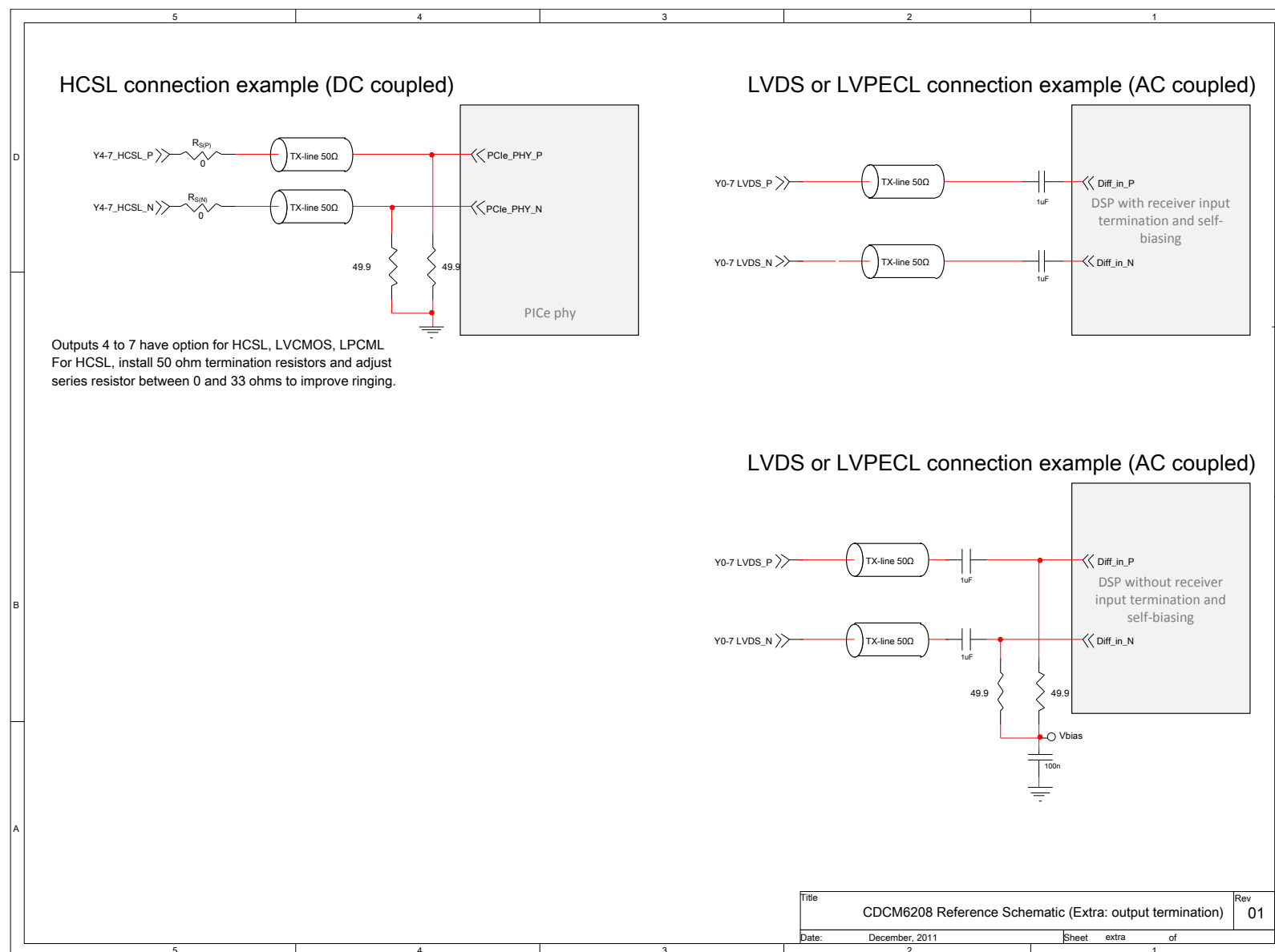
Figure 57. Schematic page 4
