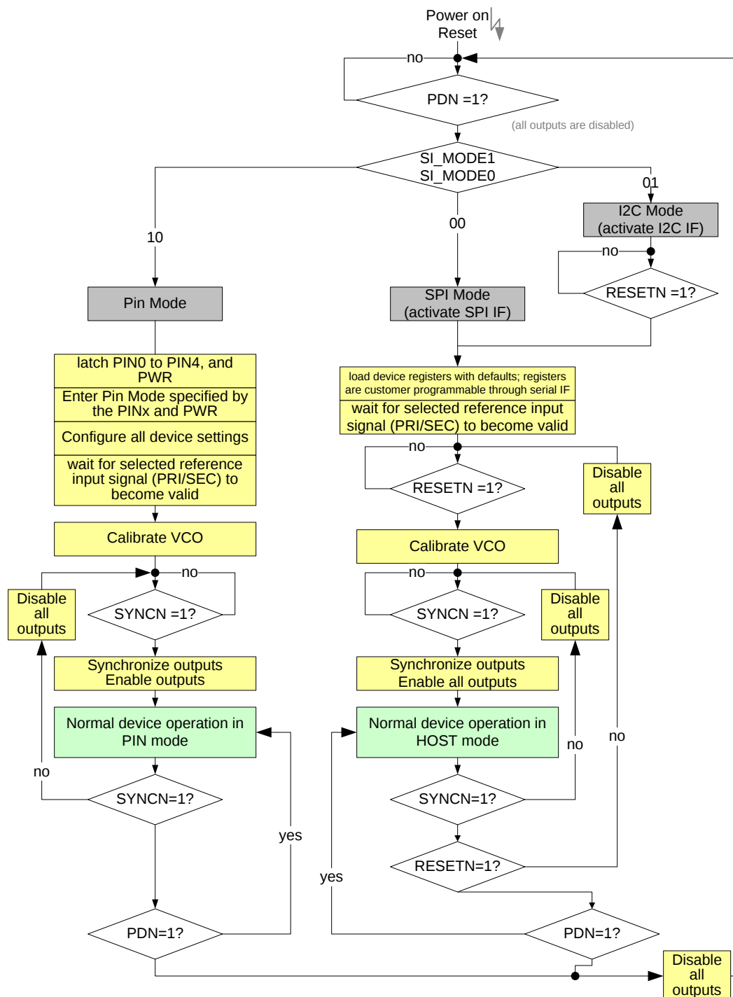
Figure 27. Device Power up and Configuration
