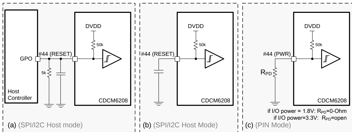
Figure 26. RESETN/PWR Pin Configurations
