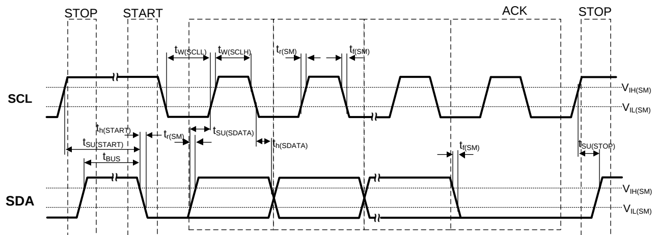
Figure 52. I 2 C Timing Diagram
