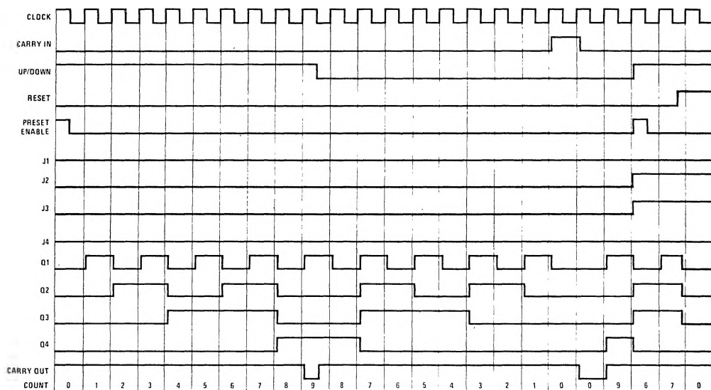
CD4510BM/CD4510BC
