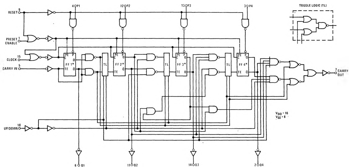
FIGURE 2. CD4516
