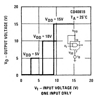
FIGURE 1. Typical Transfer Characteristics
