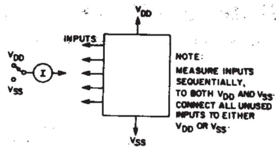
Figure 11. Input Current Test Circuit
