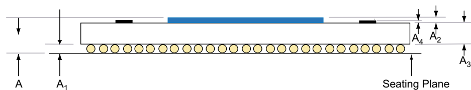
Figure 28 C-3e Network Processor BGA Package Side View
