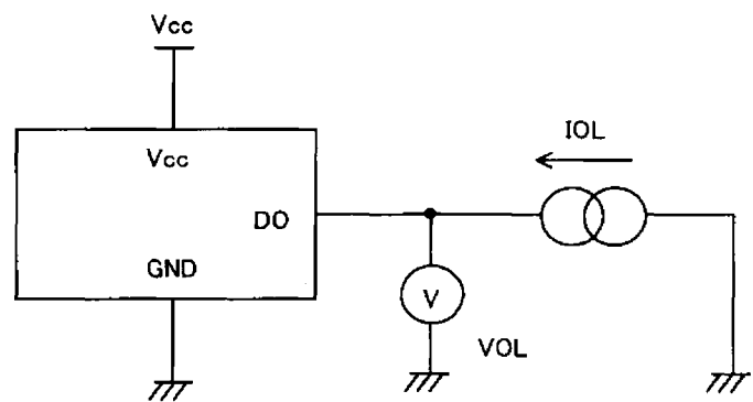
Control Output Pin to "L" Fig.-4 Output Low Voltage Test Circuit
