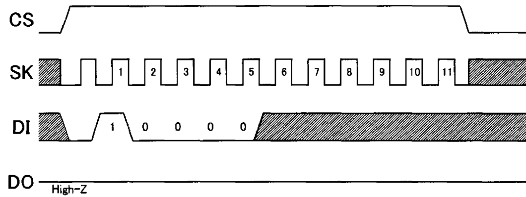
Fig.-15 Write Disable Cycle Timing
