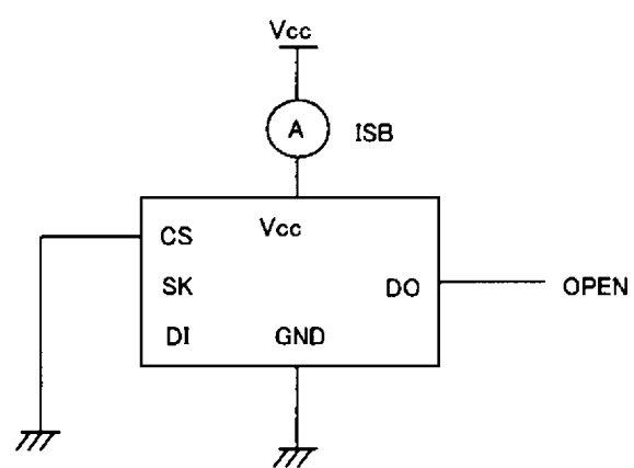
Fig.-8 Operating Current Test Circuit
