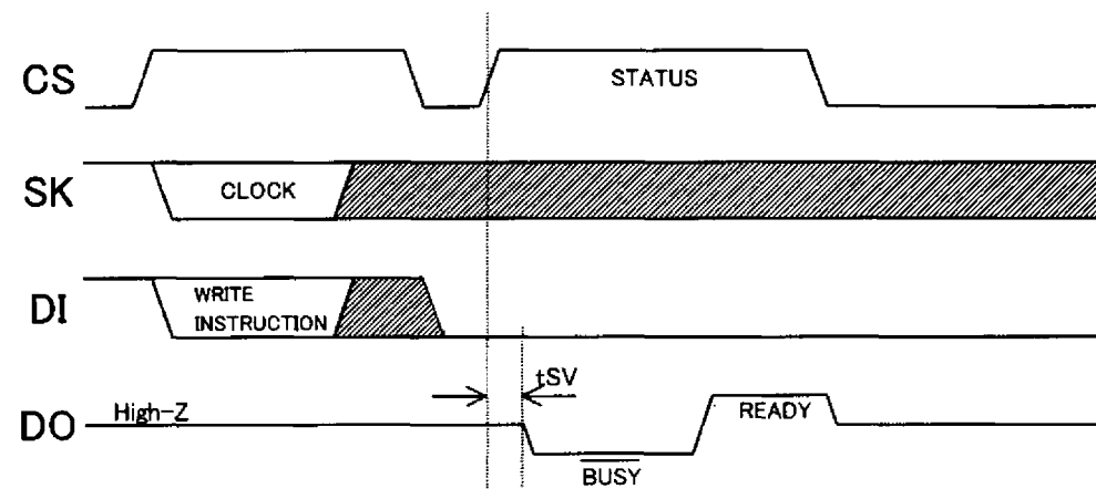
Fig.-18 READY/ \overline{\text{BUSY}} Status Output Timing
