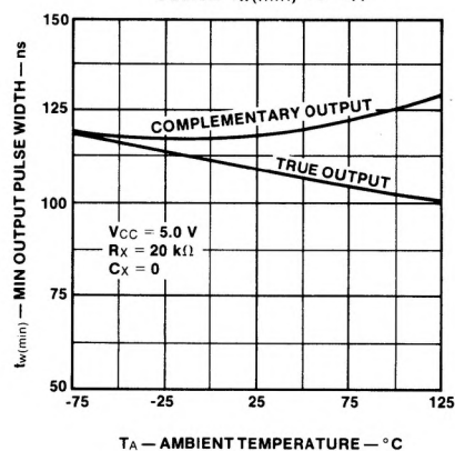
96L02 t_{w(\min)} vs T_A
