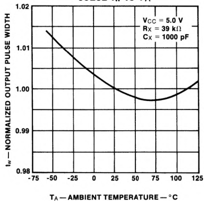
96L02 t_w vs T_A
