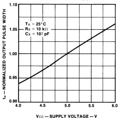
9602 t_w vs V_{CC}
