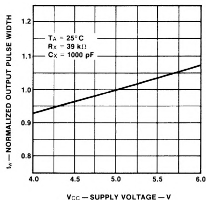
96L02 t_w vs V_{CC}
