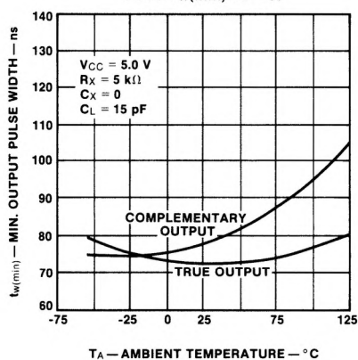
9602 t_{w(\min)} vs T_A
