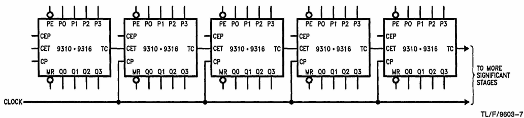
FIGURE a. Synchronous Multistage Counting Scheme (Slow)
