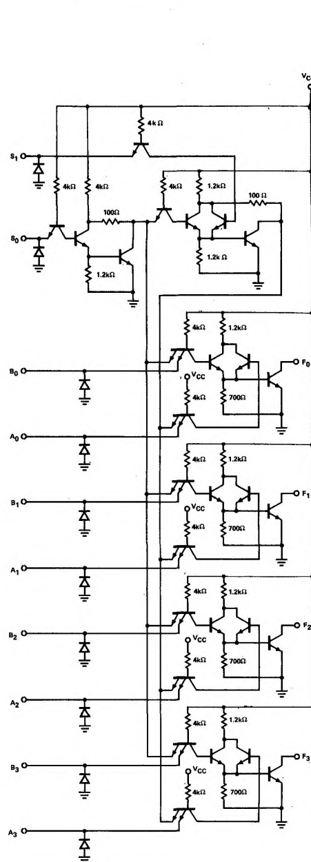
8234 (OPEN COLLECTOR)
