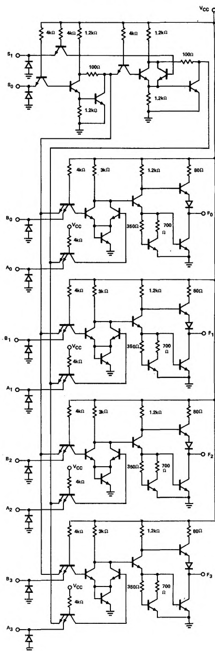
8233 (ACTIVE PULL-UP)
