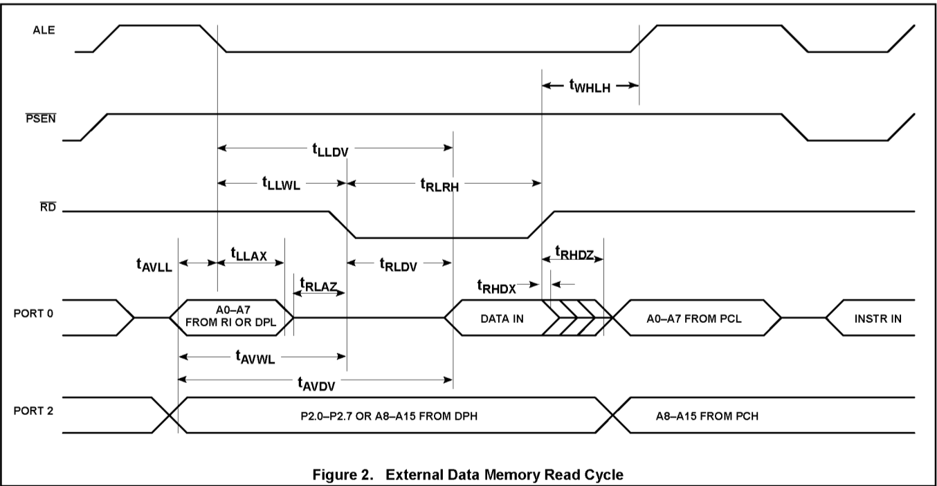
Figure 2. External Data Memory Read Cycle
