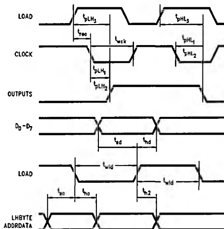
FIGURE 4. AC Specifications
