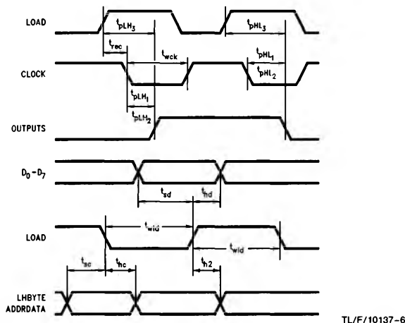
FIGURE 4. AC Specifications
